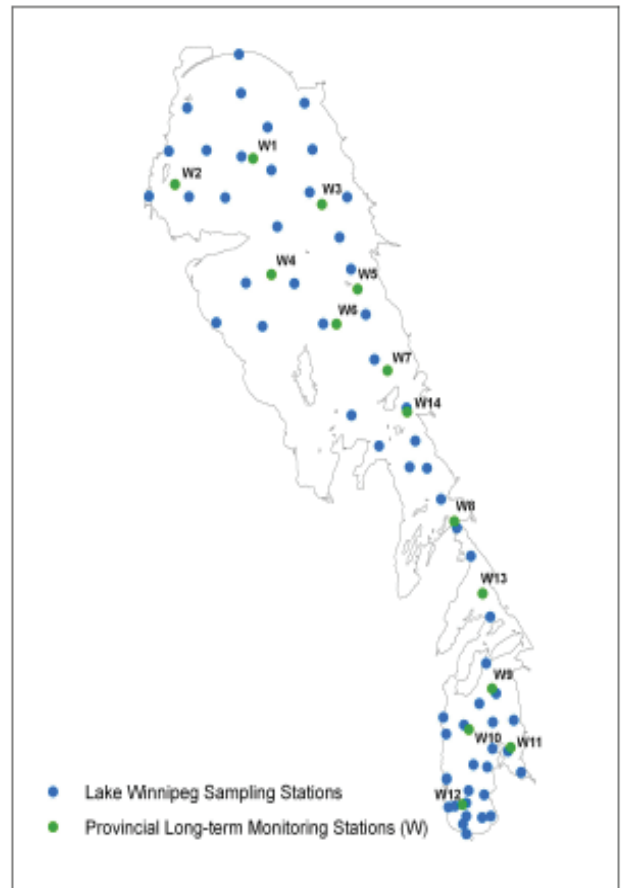
Figure 2.1: Present-day monitoring stations on Lake Winnipeg. The original network of 65 monitoring stations was selected based on those sampled in 1969; additional stations were subsequently added to the network to maximize spatial representation of the lake.
