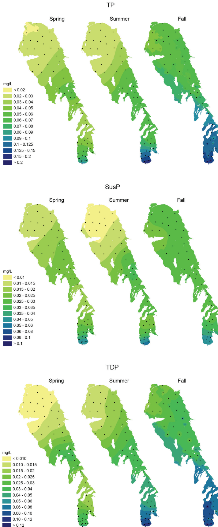
Figure 6.4: Total phosphorus, particulate phosphorus, and dissolved phosphorus in Lake Winnipeg during the spring, summer, and fall of 2002. Note the change in scale.
