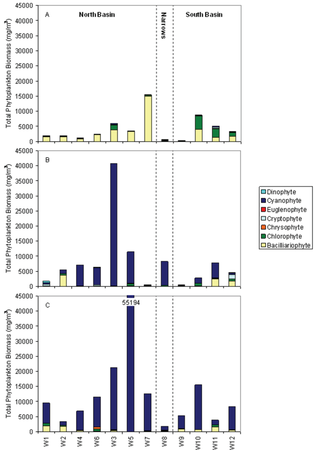
Figure 8.5: Spatial variation in total phytoplankton biomass ( \text{mg}/\text{m}^3 ) and community composition at the 12 long-term stations located in the north basin, narrows, and south basin of Lake Winnipeg during the spring (A), summer (B), and fall (C) monitoring periods of 2006.
