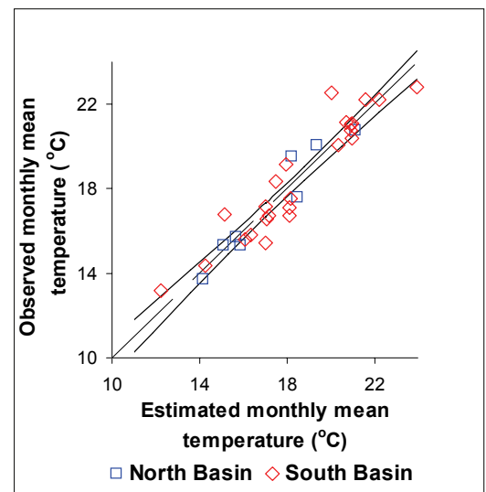
Figure A1. Comparison of modelled with observed monthly mean surface water temperature, where observed monthly means were calculated from the 10-minute interval record at moorings in the north and south basins. Solid lines indicate 95 % confidence limits for the mean prediction; dashed line indicates target 1:1 prediction of observed temperature. Model-building data were obtained from ship-board measurements made on six whole-lake cruises in 1969. Validation data are from the period 1999 to 2006.
