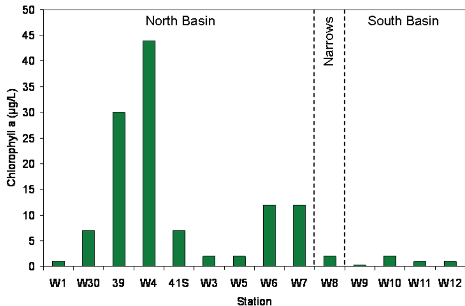
Figure 8.7: Chlorophyll a concentrations (µg/L) measured at 14 stations during the under-ice period (January-April), 2007.
