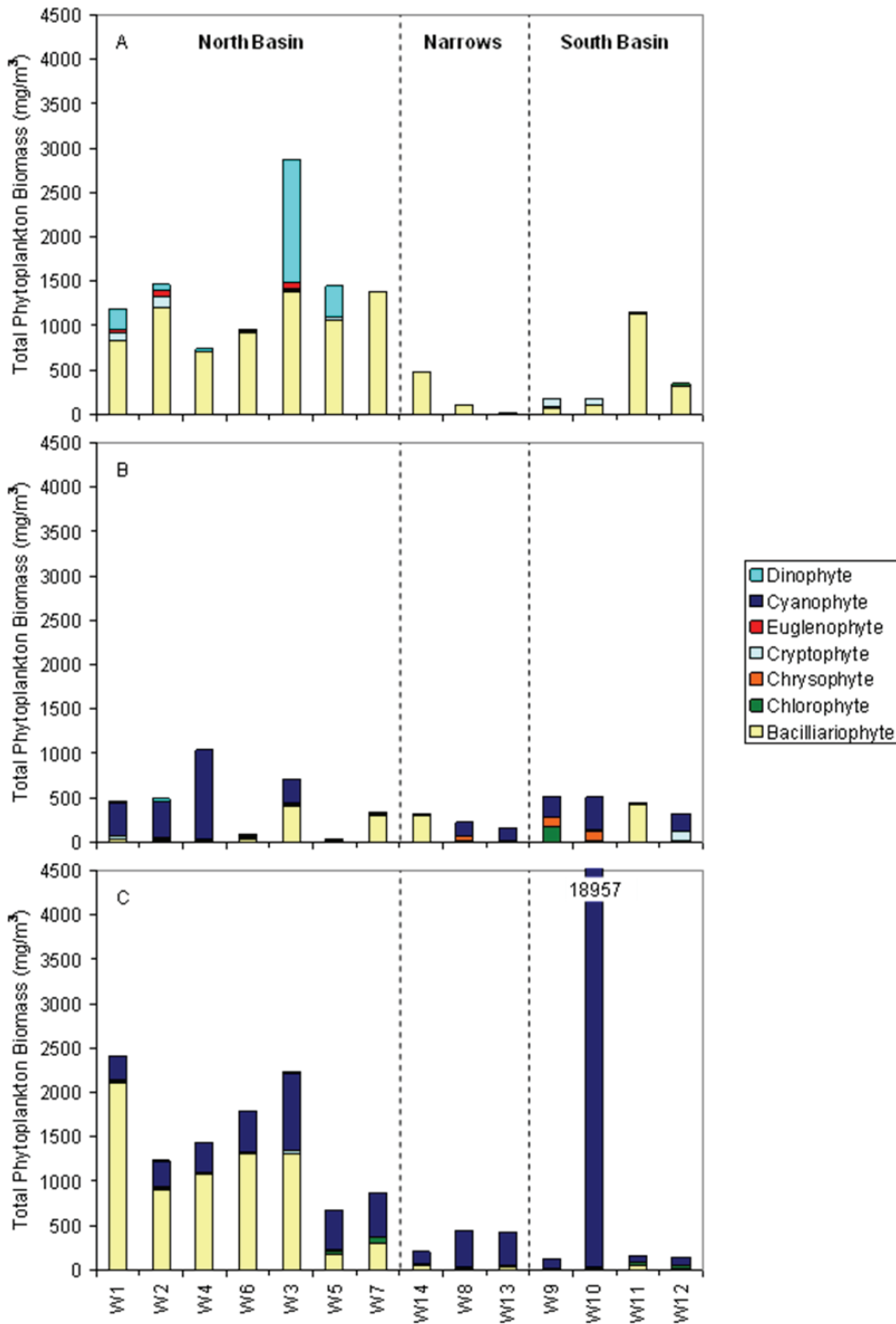
Figure 8.6: Spatial variation in total phytoplankton biomass ( \text{mg}/\text{m}^3 ) and community composition at the 14 long-term stations located in the north basin, narrows, and south basin of Lake Winnipeg during the spring (A), summer (B), and fall (C) monitoring periods of 2007.
