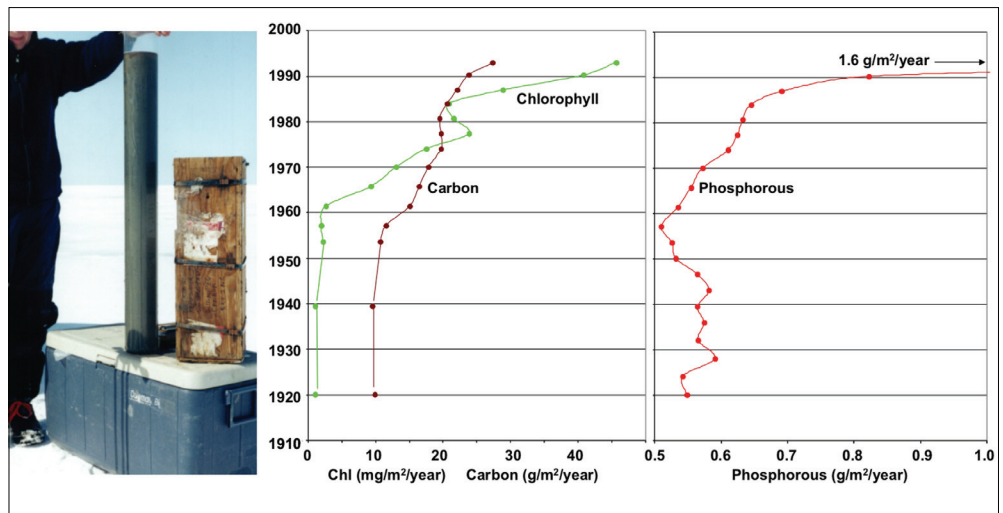
Figure 9.3: Phosphorus, (P), carbon (C) and chlorophyll measured in 1994 core from the central north basin of Lake Winnipeg. Note increased deposition since the late 1950s, coincident with increased agricultural practices in the watershed, hydro-electric development, and impoundment of the Saskatchewan River since early 1960s and lake level regulation since 1976.
