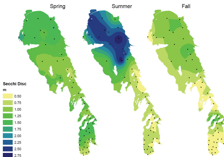
Figure 5.20: Secchi disc depths in Lake Winnipeg surface waters over the spring (May-June), summer (July-August), and fall (September-October) of 2002.
