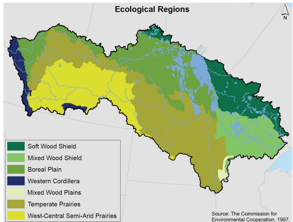
Figure 3.6a: Ecological regions. (Data Source: Commission for Environmental Cooperation 1997)
