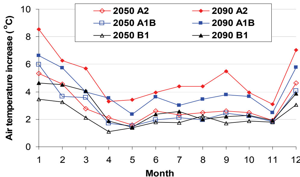
Figure 9.16: Increases in air temperature predicted for the Lake Winnipeg region for two 20-year periods, 2040 to 2059 (labelled 2050) and 2080 to 2099 (labelled 2090) using CGCM3 with 3 forcing emissions scenarios, B1, A1B, and A2. Each point is the mean of 100 predicted values, i.e. 5 model runs X 20 years. Predicted 21 st century temperatures are compared to temperatures modelled using CGCM3 over the base period from 1970 to 1992 (excluding the years 1976, 1980, and 1981 for which considerable data is missing in the observed record).
