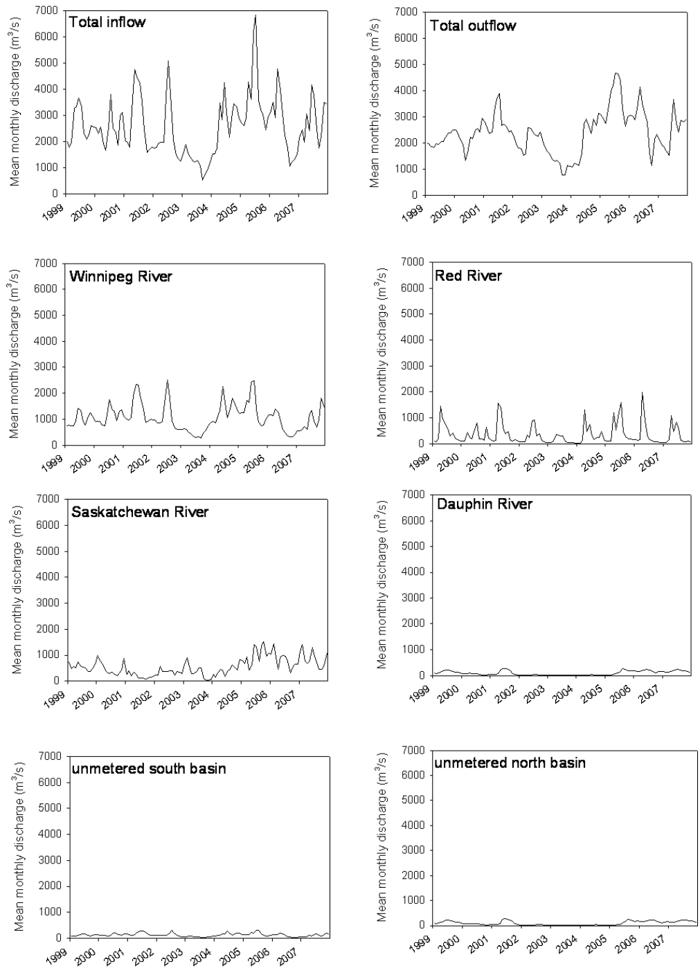
Figure 4.5: Mean monthly discharges to and from Lake Winnipeg 1999 to 2007. (Data Source: Water Survey of Canada; G. McCullough)
