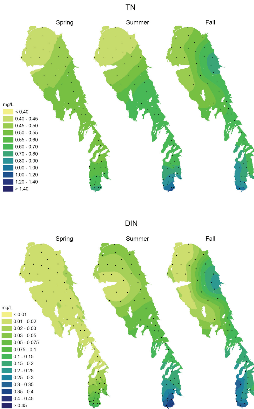
Figure 6.8: Total nitrogen and dissolved inorganic nitrogen in Lake Winnipeg during the spring, summer, and fall of 2002.
