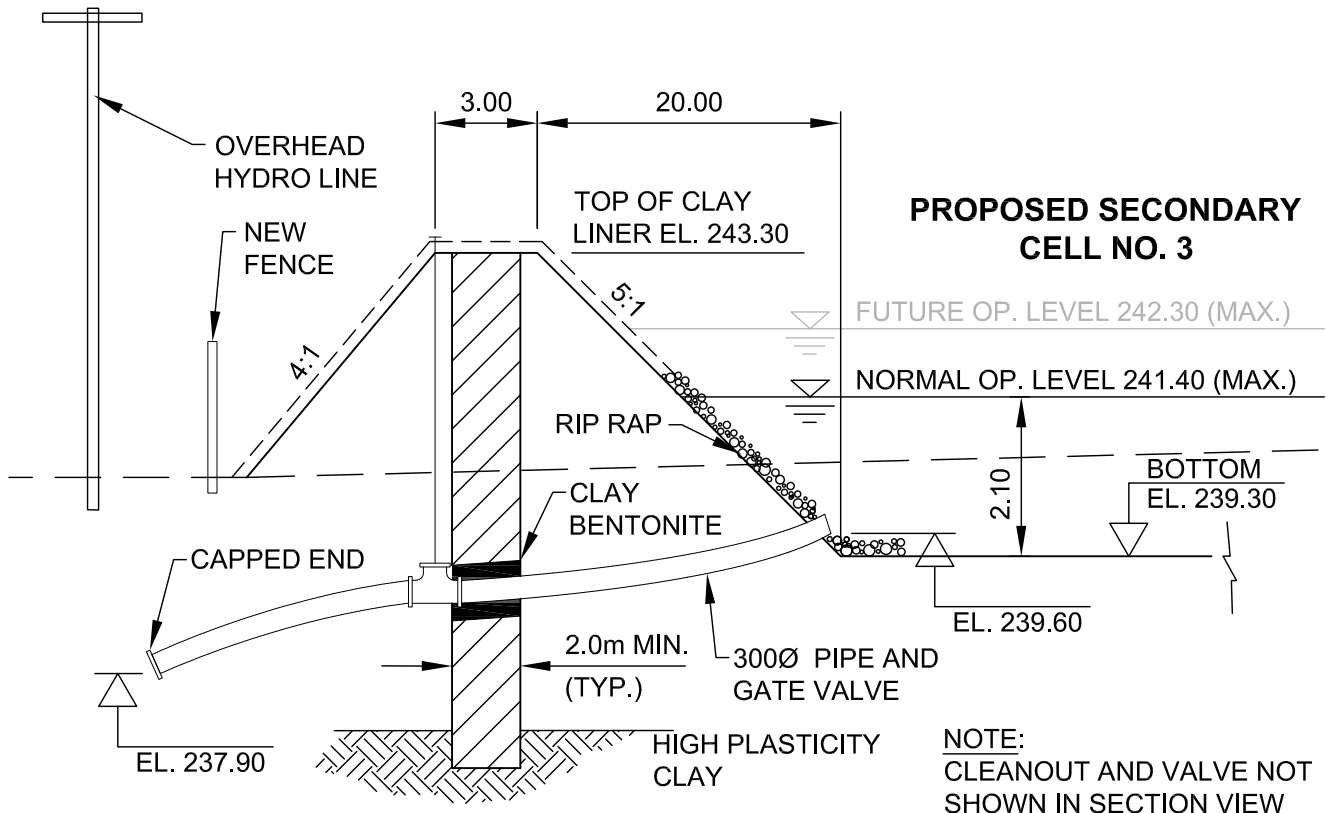
2 PROPOSED PIPE INSTALLATION - SECTION VIEW N.T.S.
