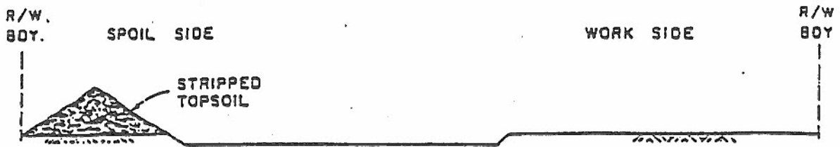
1. TOPSOIL STRIPPED
