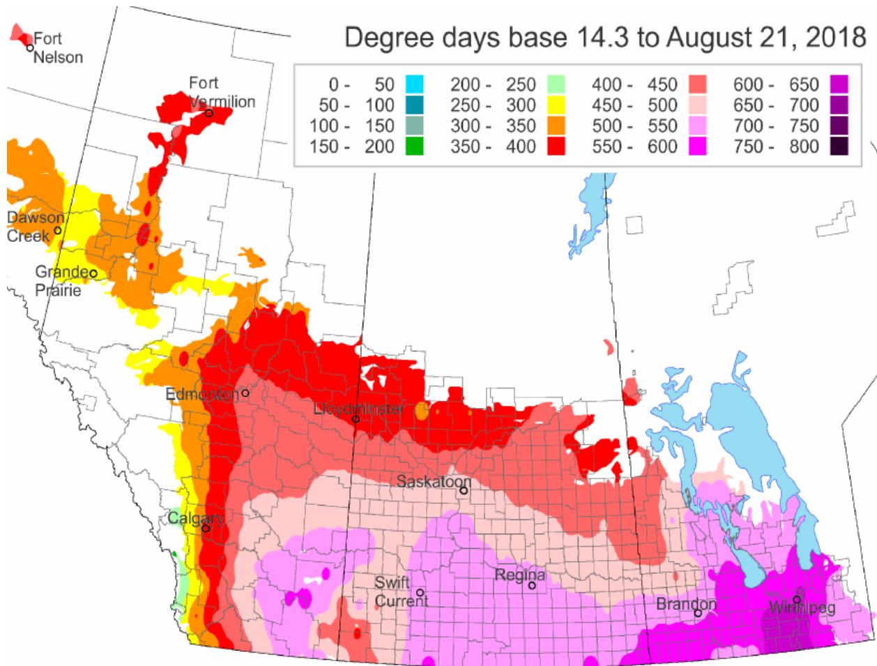
Figure 4 - Degree day accumulations, as of Week 33, across the Prairie Provinces
