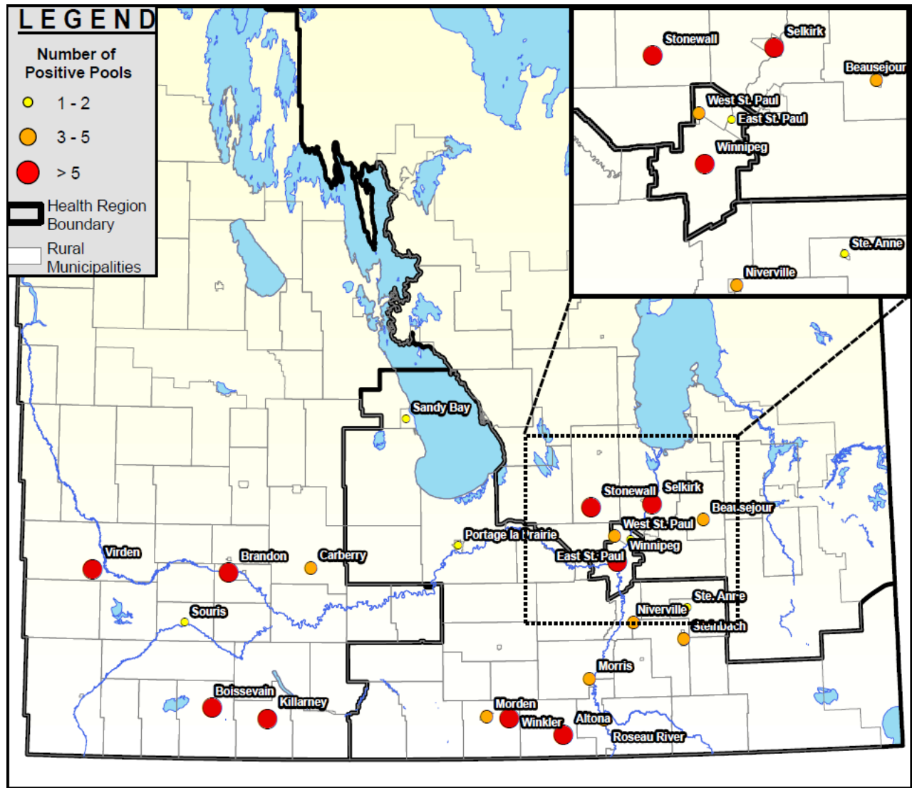
Figure 3 – Distribution of WNV positive Culex tarsalis mosquito pools collected in southern Manitoba (current to Week 33).
