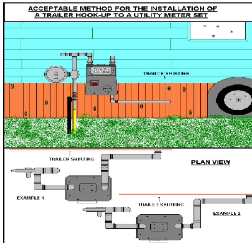
Figure 1 Piped connections to manufactured homes
